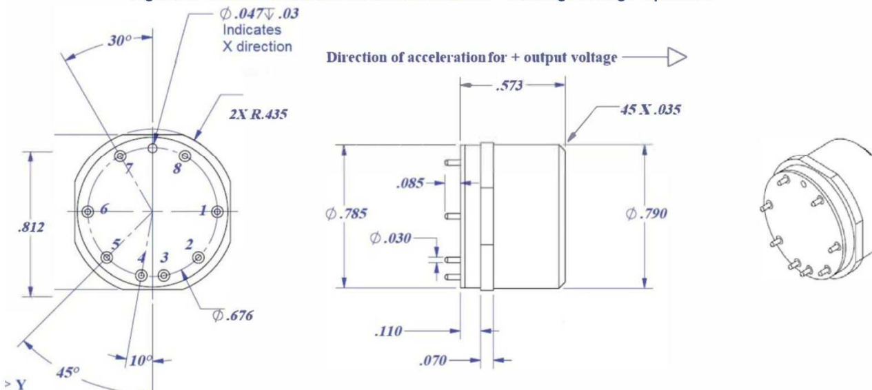
Figure 2. Model 60 MicroAcc Accelerometer - Package Design Option B
