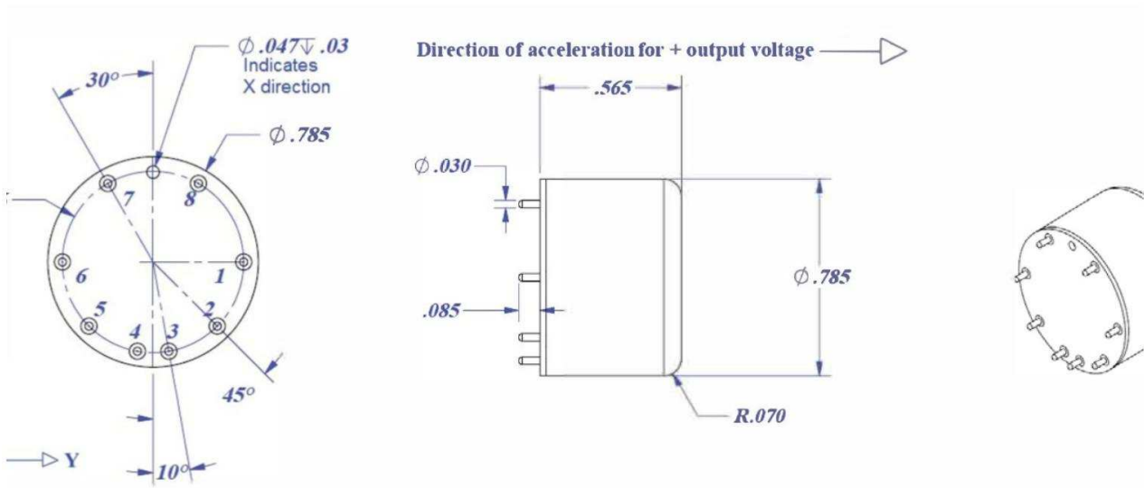
Figure 1. Model 60 MicroAcc Accelerometer - Package Design Option A
